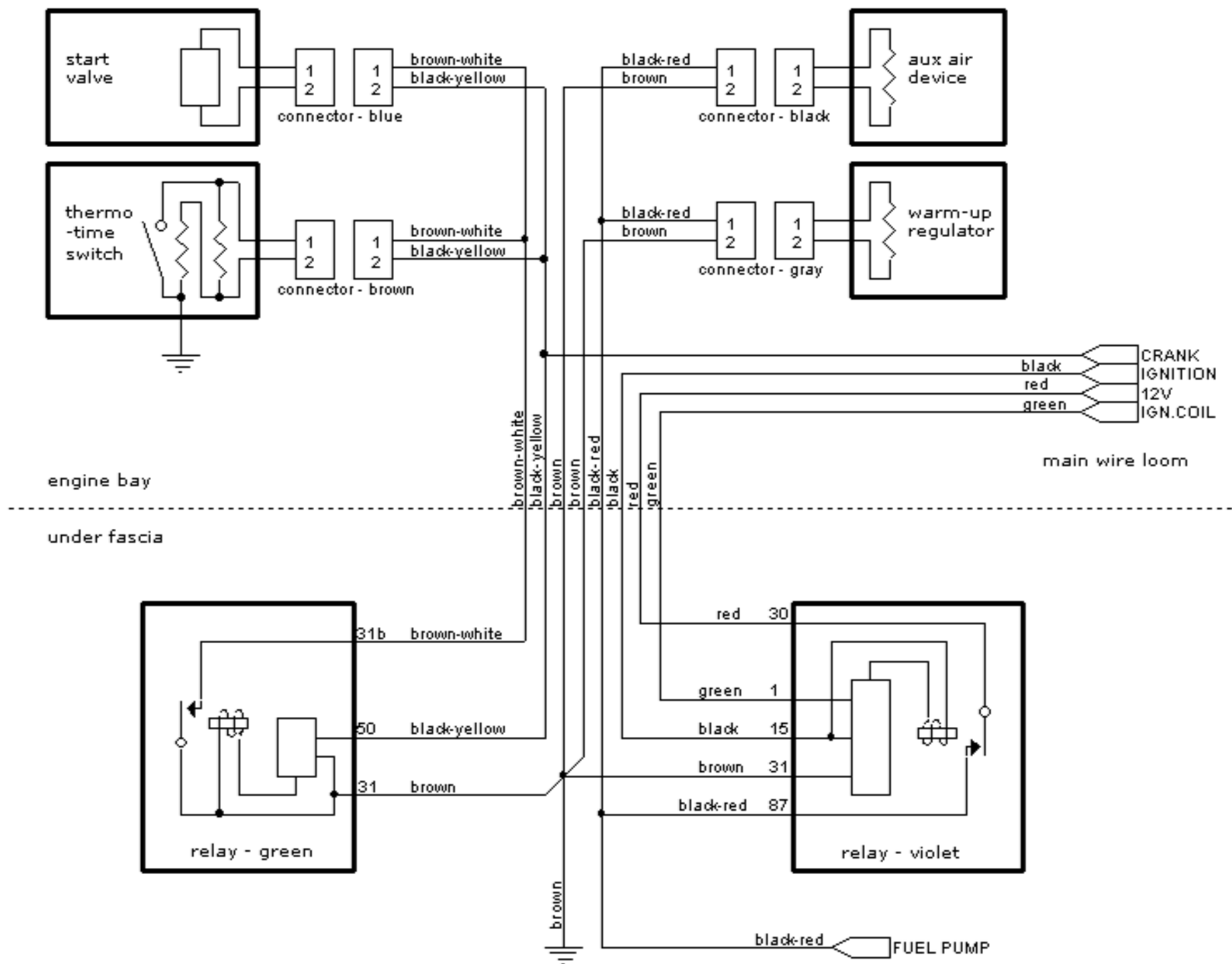
Ford Capri 2.8i - K-Jetronic wiring diagram
